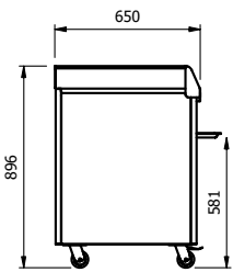
Model VCCSB
