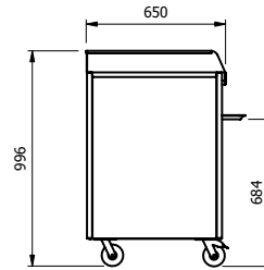
Model VCCS
