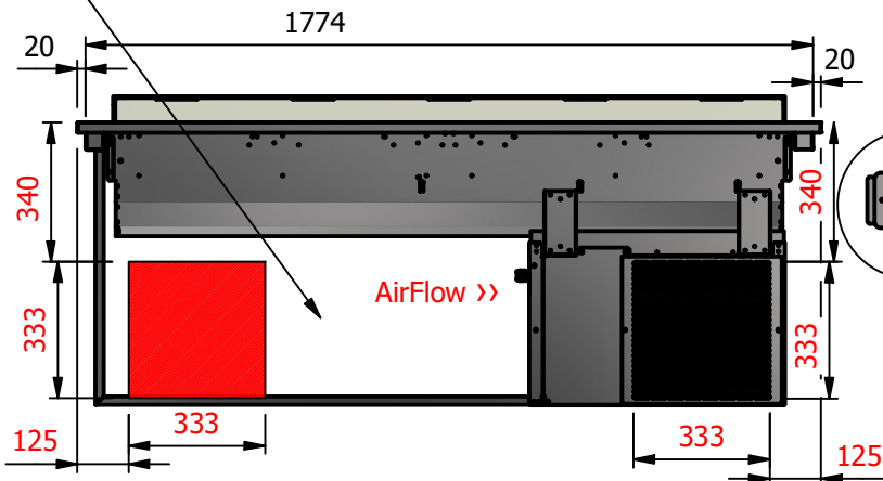
Rear View [Operators Side]
