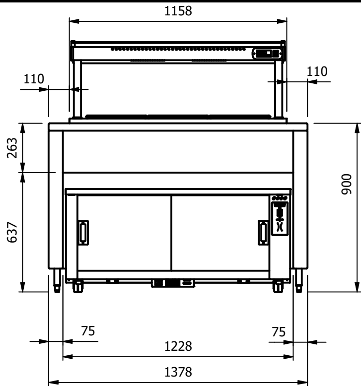
Typical Counter Installation HC3R with Size 3 Drop In unit
