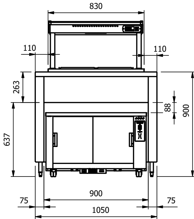
Typical Counter Installation HC2R with Size 2 Drop In unit
